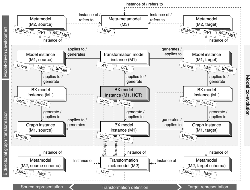
Figure 2: Overview of our model co-evolution approach.
